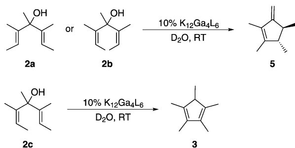
Scheme 3. In unbuffered \text{D}_2\text{O} at room temperature, the 1 -catalyzed Nazarov reaction of symmetrical substrates 2a and 2b produces 5 , while the reaction of 2c forms \text{Cp}^*\text{H}.
